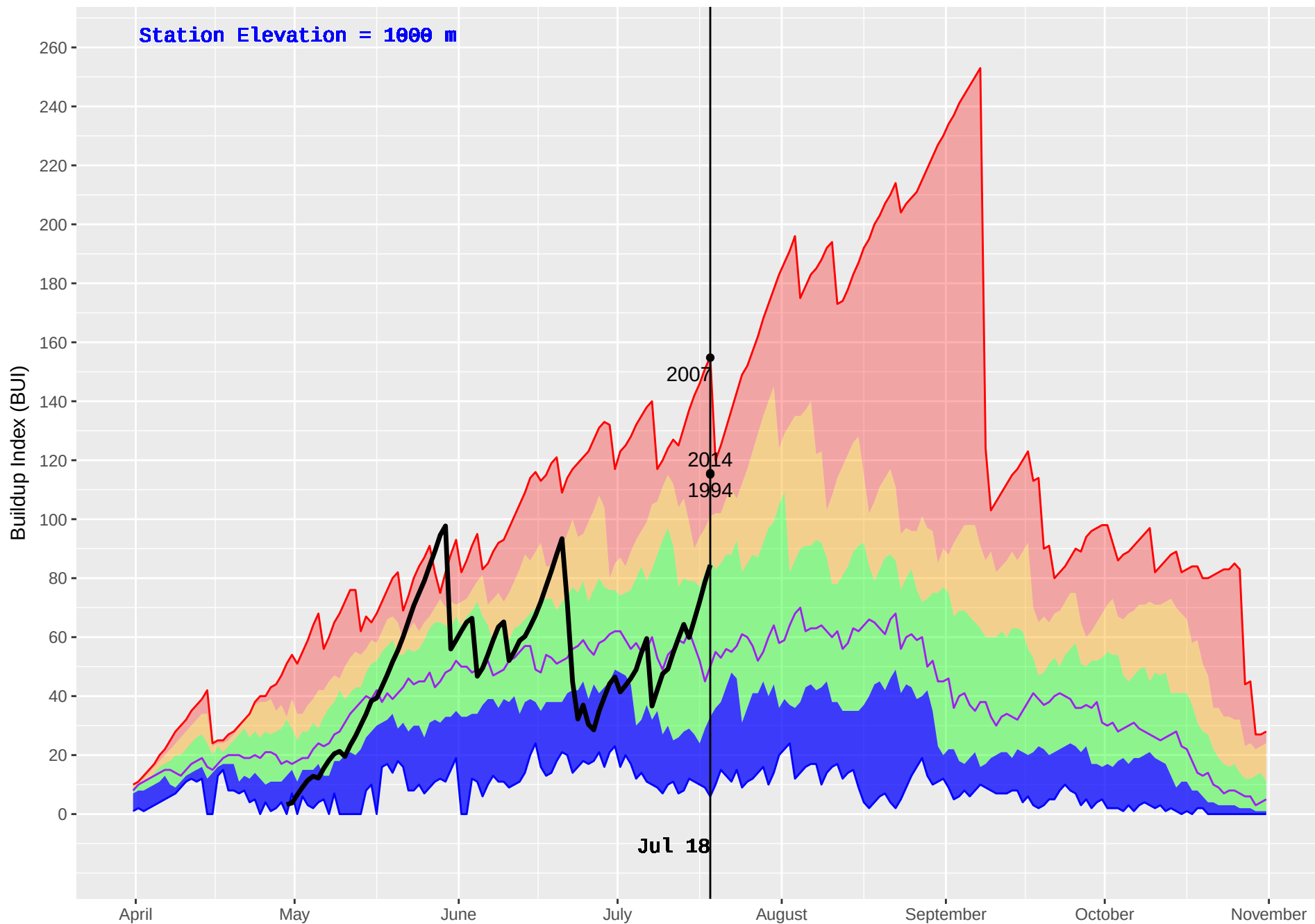
SUCCOUR CREEK (374) : Historical (1986–2016) and Current (2018) Daily Buildup Index (BUI)
